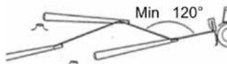
6.1.1 Minimum angle for herringbone pattern
