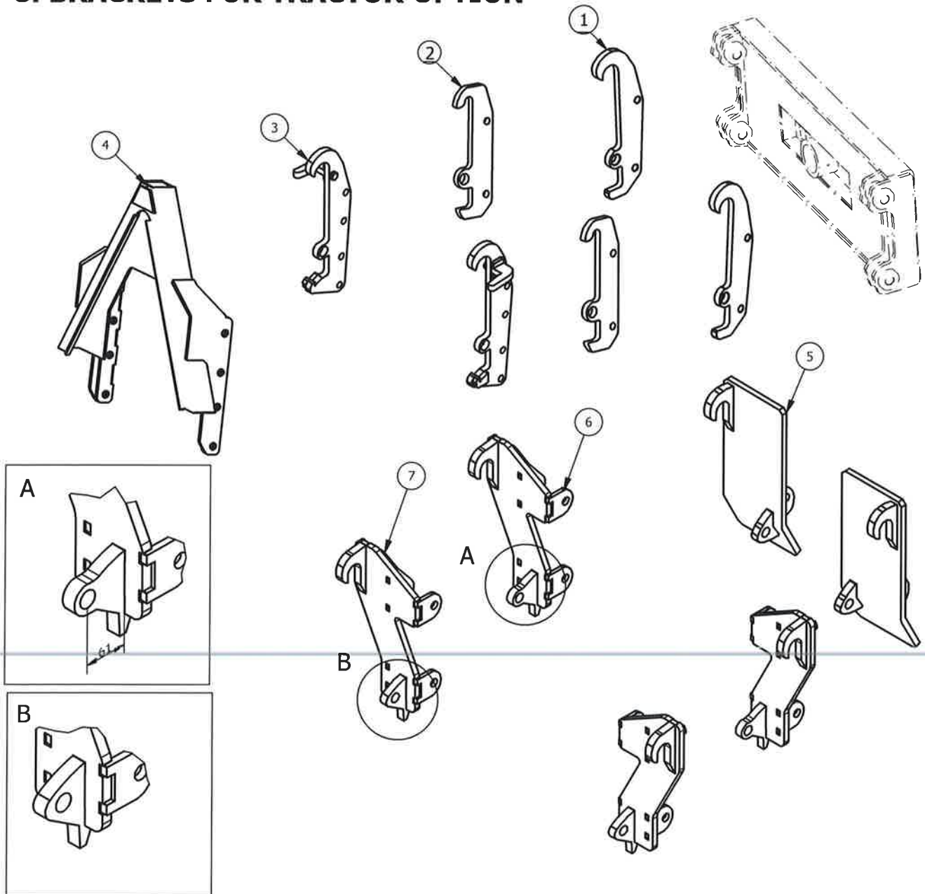
RESERVEDELSLISTE – SPARE PARTS LIST
