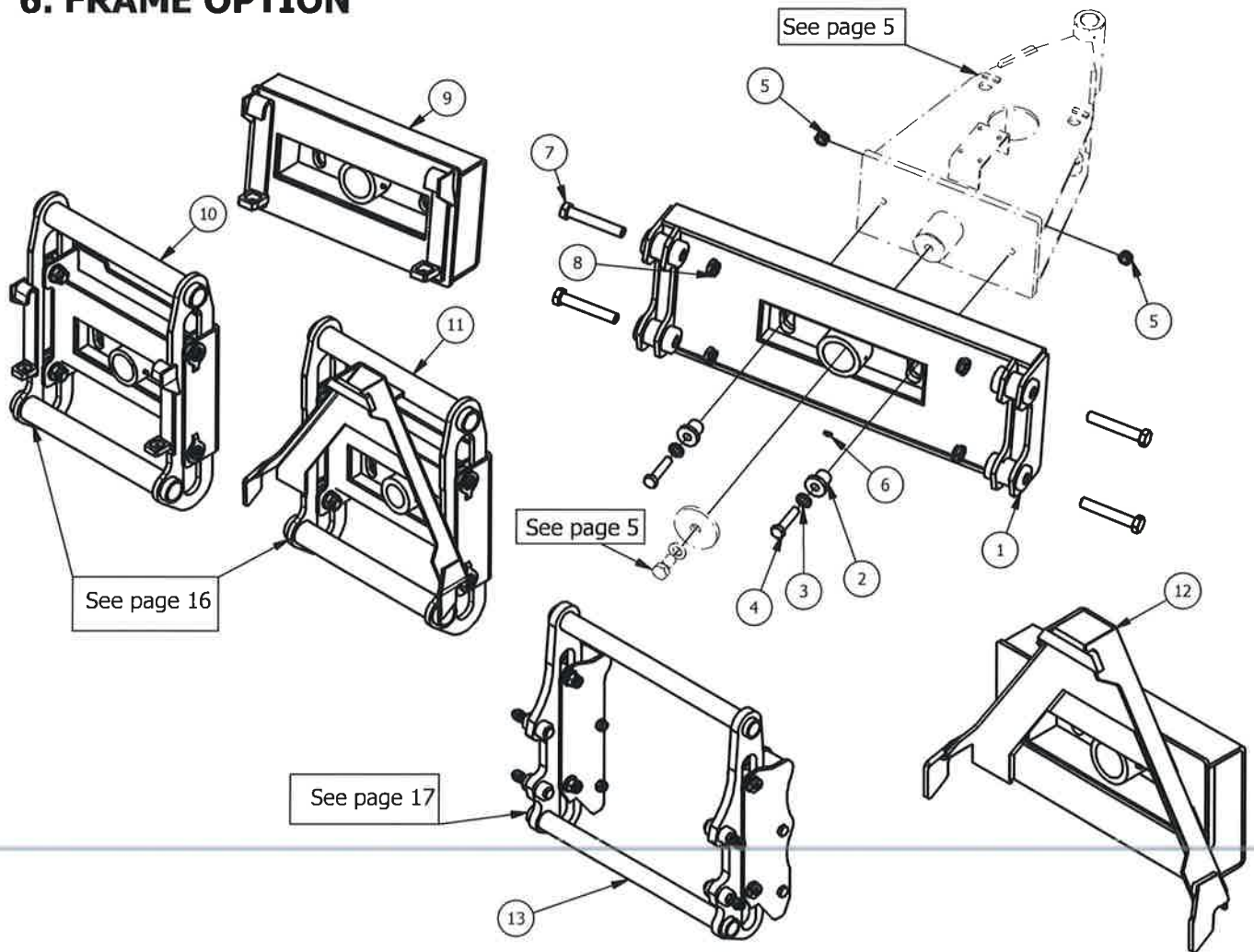
RESERVEDELSLISTE – SPARE PARTS LIST
